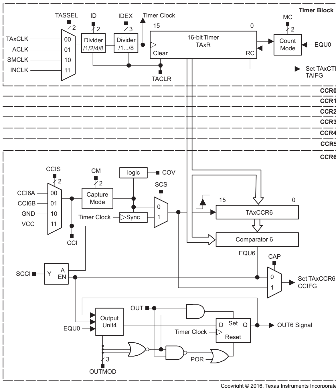
Figure 13-1. Timer_A Block Diagram
