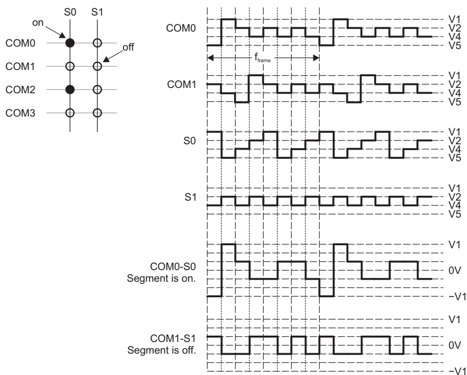
Figure 17-15. Example 4-Mux Waveforms
