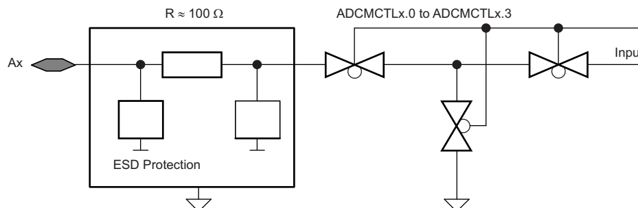
Figure 21-2. Analog Multiplexer
