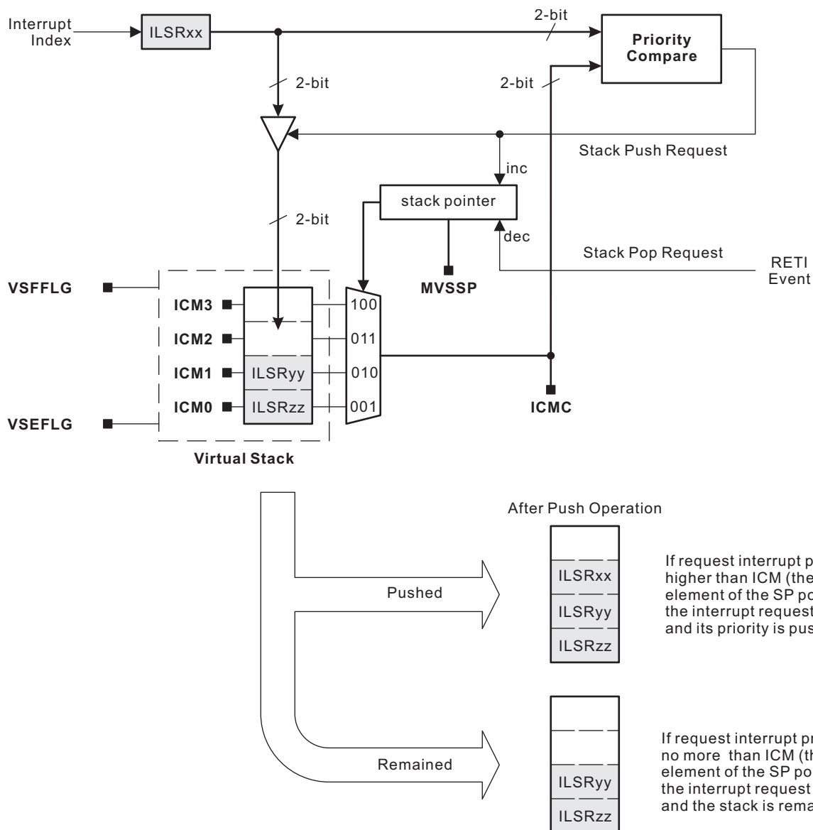
Figure 5-3. Virtual Stack Push Flow Block Diagram
