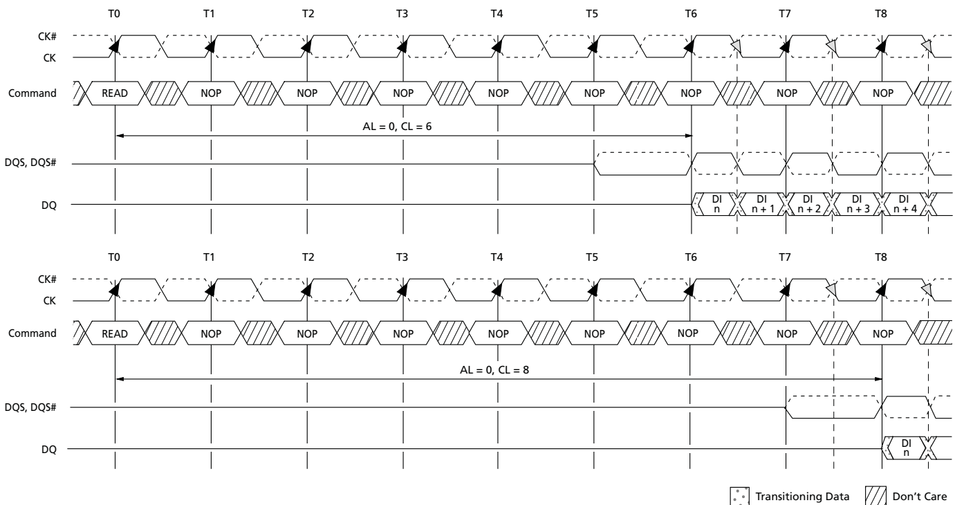
Figure 52: READ Latency
