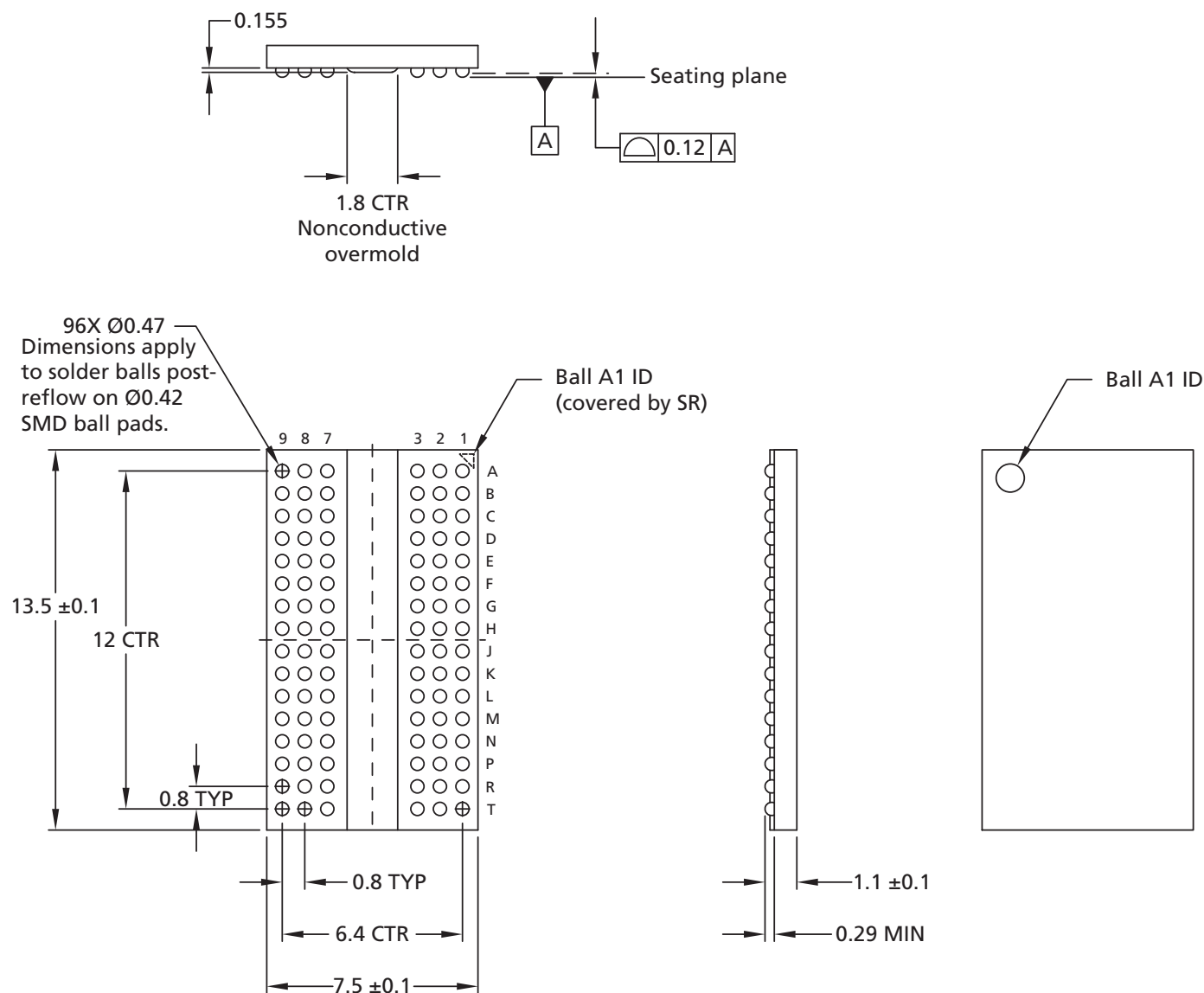
Figure 12: 96-Ball FBGA – x16 (LY)
