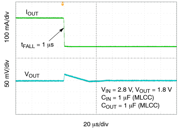
Figure 45. Load Transient Response – 250 mA to 1 mA – V_{OUT} = 1.8 V
