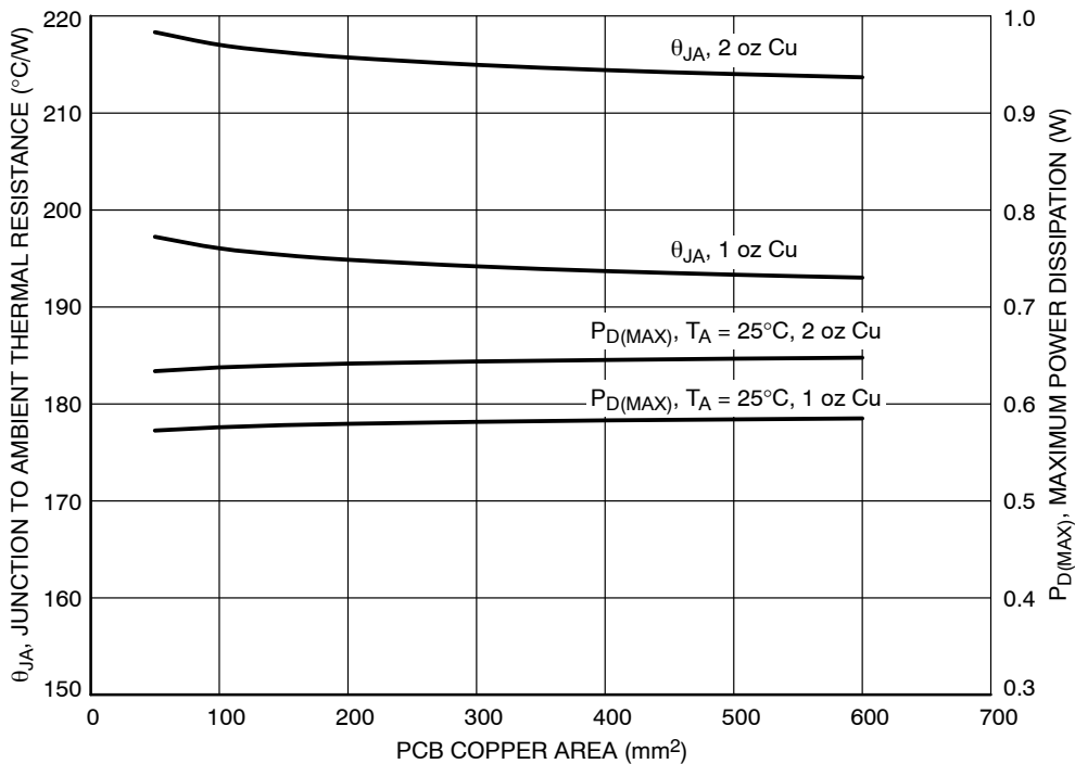
Figure 54. \theta_{JA} and P_{D(MAX)} vs. Copper Area (XDFN4)
