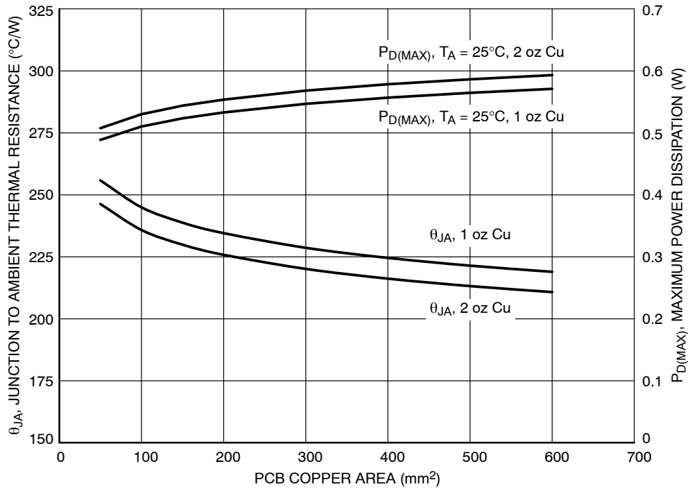
Figure 52. \theta_{JA} and P_{D(MAX)} vs. Copper Area (SOT23-5L)
