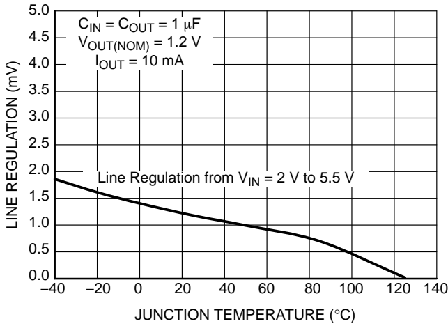
Figure 30. Line Regulation vs. Temperature V_{OUT} = 1.2\text{ V}
