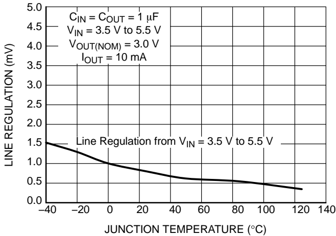
Figure 34. Line Regulation vs. Temperature V_{OUT} = 3.0\text{ V}
