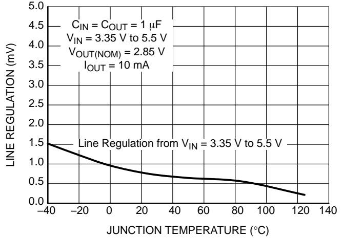
Figure 33. Line Regulation vs. Temperature V_{OUT} = 2.85\text{ V}
