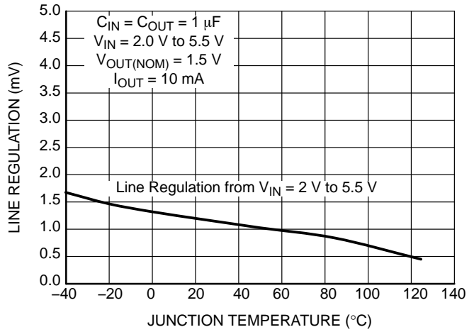
Figure 31. Line Regulation vs. Temperature V_{OUT} = 1.5\text{ V}
