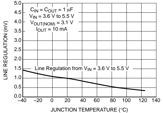
Figure 35. Line Regulation vs. Temperature V_{OUT} = 3.1\text{ V}
