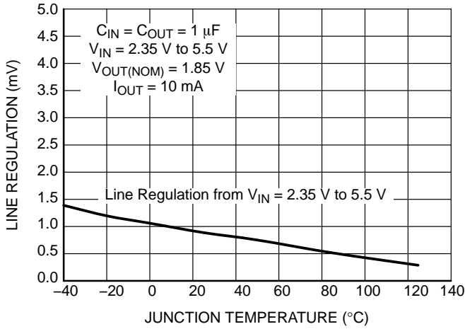
Figure 32. Line Regulation vs. Temperature V_{OUT} = 1.85\text{ V}
