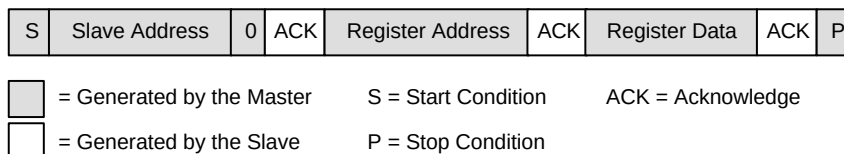
Figure 11. Single Register Write Operation
