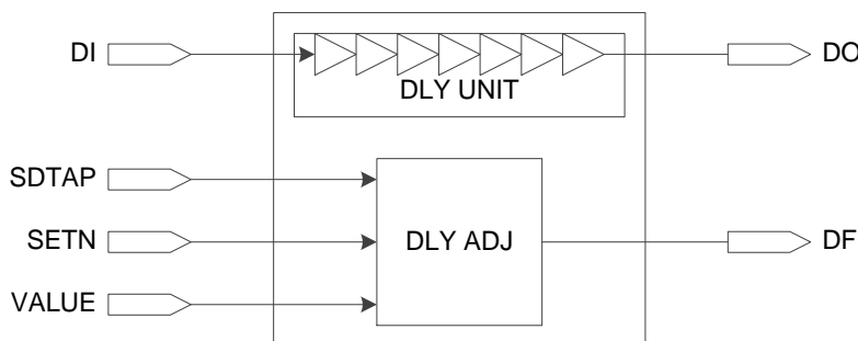
Figure 2-10 IODELAY Diagram
