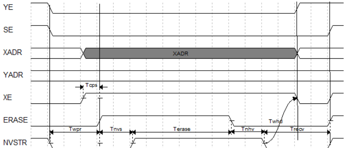
Figure 3-3 Erase Timing
