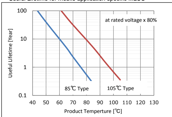
Useful Lifetime for mobile application specific MLCC
