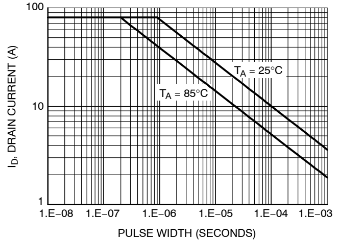
Figure 16. Avalanche Characteristics
