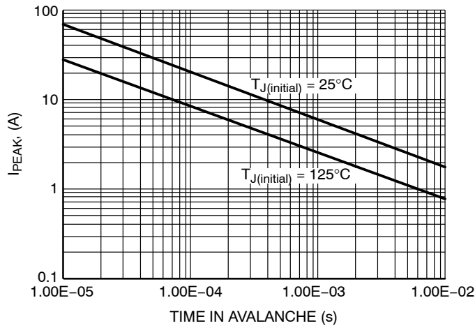
Figure 13. Avalanche Characteristics
