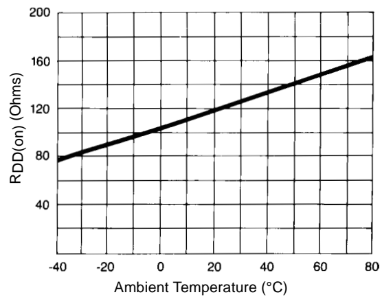
Figure 4. Typical On-Resistance
