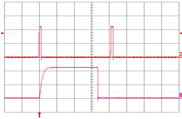
Figure 3.3V.24. Load current (top trace, 20 A/div., 50 ms/div.) into a 10 \text{ m}\Omega short circuit during restart, at V_{in} = 48 \text{ V} . Bottom trace (20 A/div., 2 ms/div.) is an expansion of the on-time portion of the top trace.
