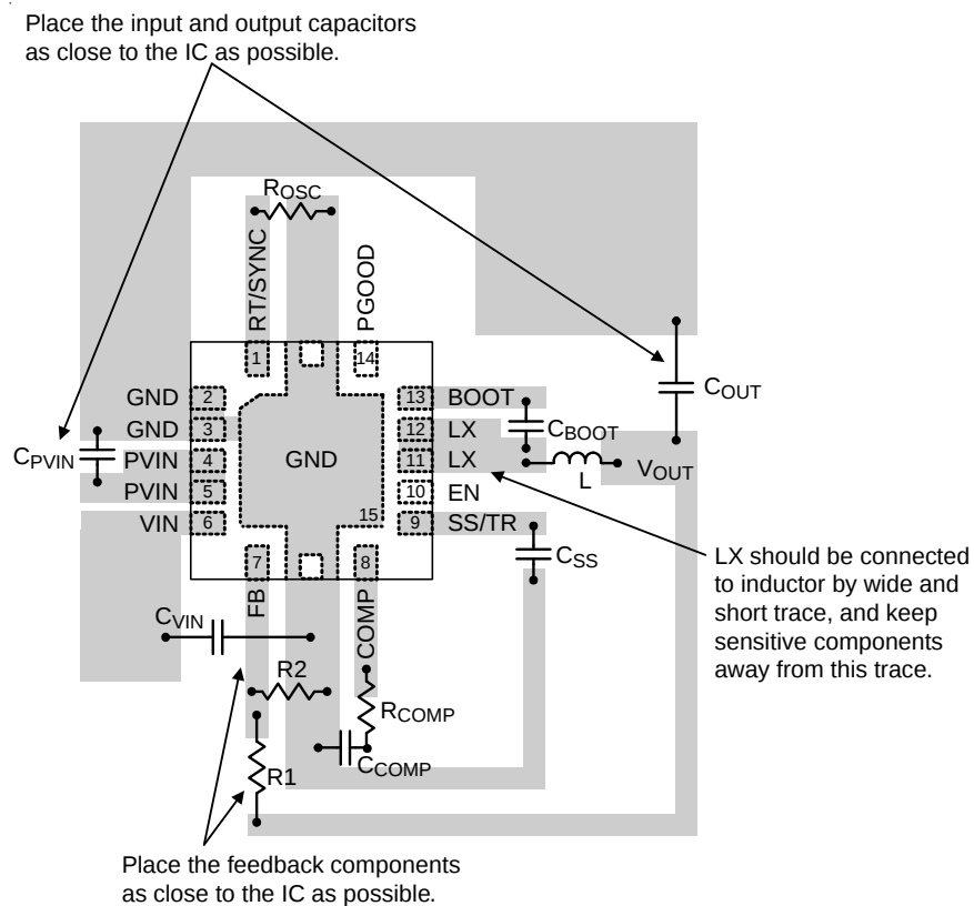
Figure 11. PCB Layout Guide
