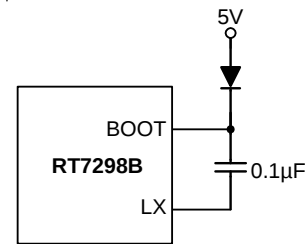
Figure 9. External Bootstrap Diode
