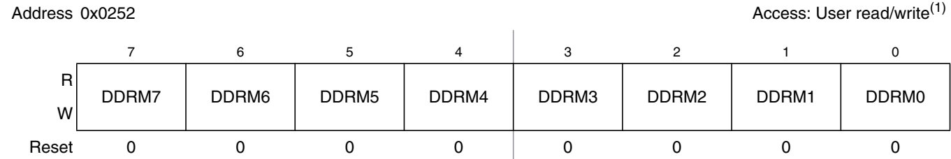
Figure 2-37. Port M Data Direction Register (DDRM)
