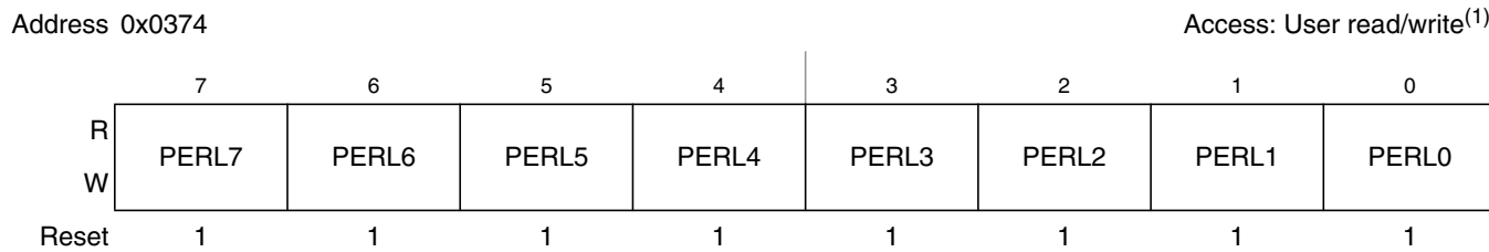
Figure 2-95. Port L Pull Device Enable Register (PERL)
