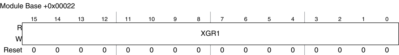
Figure 10-15. XGATE Register 1 (XGR1)
