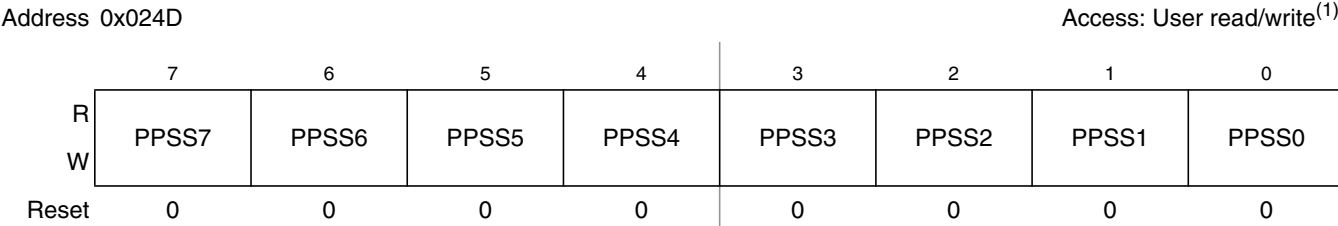
Figure 2-32. Port S Polarity Select Register (PPSS)
