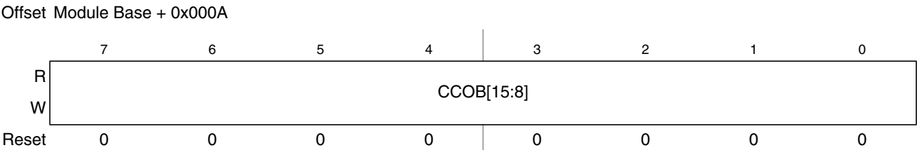
Figure 26-16. Flash Common Command Object High Register (FCCOBHI)
