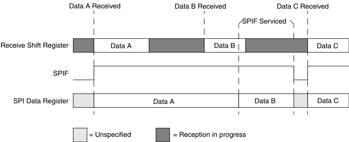
Figure 21-9. Reception with SPIF serviced in Time
