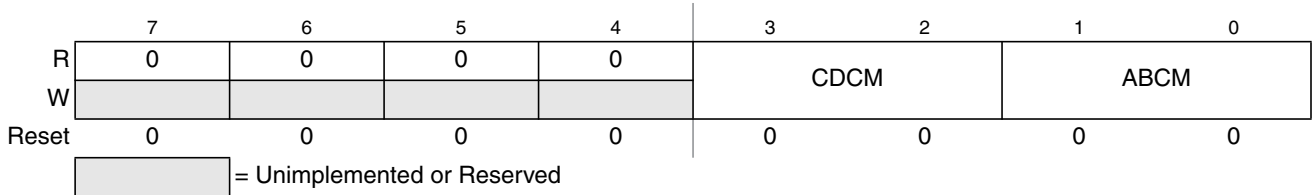
Figure 8-6. Debug Control Register2 (DBG2)
