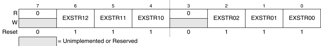
Figure 5-4. External Bus Interface Control Register 1 (EBICTL1)
