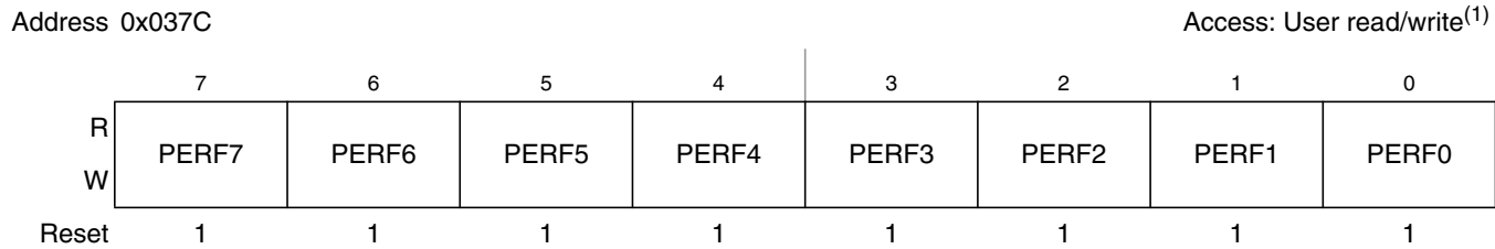
Figure 2-103. Port F Pull Device Enable Register (PERF)
