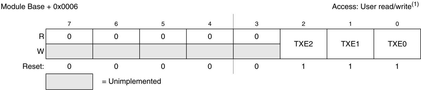
Figure 16-10. MSCAN Transmitter Flag Register (CANTFLG)
