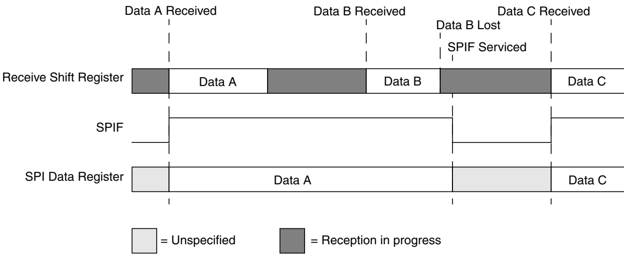
Figure 21-10. Reception with SPIF serviced too late
