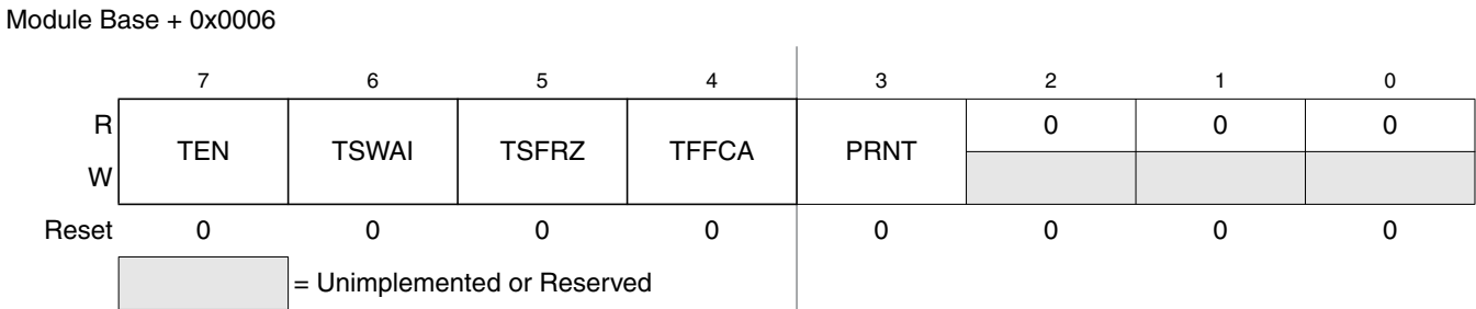
Figure 22-12. Timer System Control Register 1 (TSCR1)
