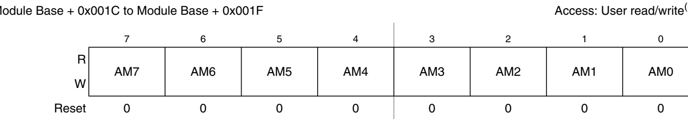
Figure 16-23. MSCAN Identifier Mask Registers (Second Bank) — CANIDMR4–CANIDMR7
