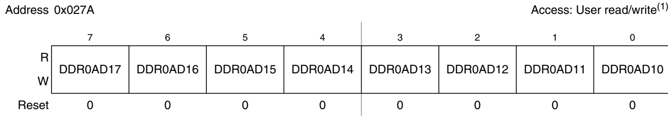
Figure 2-77. Port AD1 Data Direction Register 0 (DDR0AD1)
