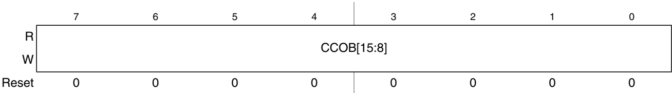
Figure 24-16. Flash Common Command Object High Register (FCCOBHI)
