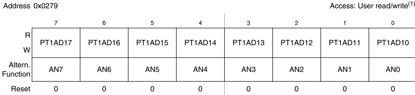
Figure 2-76. Port AD1 Data Register 1 (PT1AD1)
