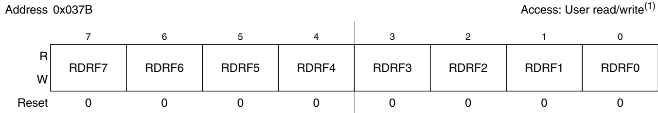
Figure 2-102. Port F Reduced Drive Register (RDRF)
