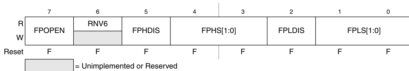
Figure 26-13. Flash Protection Register (FPROT)
