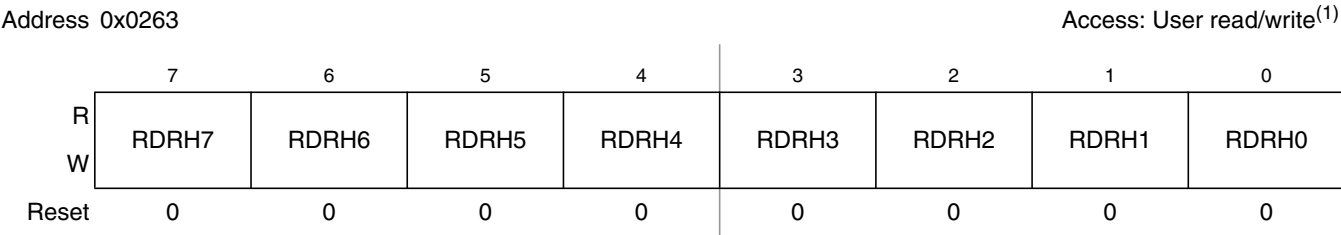
Figure 2-54. Port H Reduced Drive Register (RDRH)
