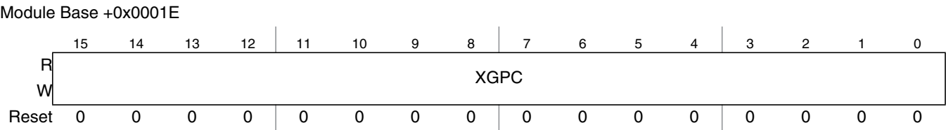
Figure 10-14. XGATE Program Counter Register (XGPC)
