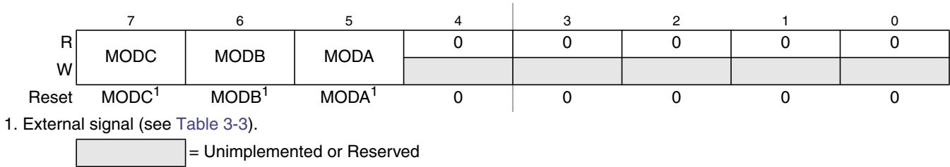
Figure 3-4. Mode Register (MODE)
