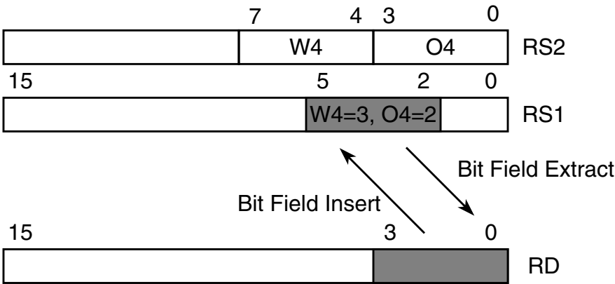
Figure 10-26. Bit Field Addressing
