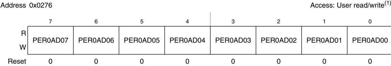
Figure 2-73. Port AD0 Pull Device Up Register 0 (PER0AD0)
