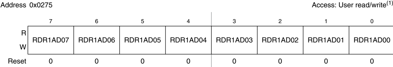
Figure 2-72. Port AD0 Reduced Drive Register 1 (RDR1AD0)
