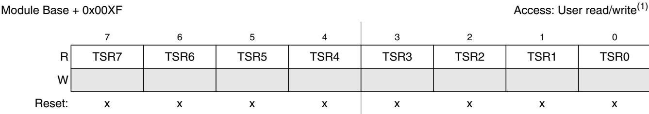
Figure 16-38. Time Stamp Register — Low Byte (TSRL)
