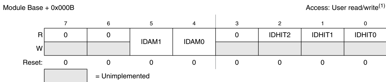
Figure 16-15. MSCAN Identifier Acceptance Control Register (CANIDAC)
