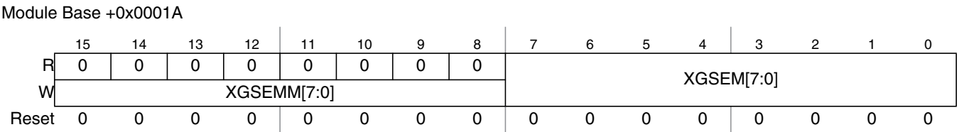
Figure 10-12. XGATE Semaphore Register (XGSEM)
