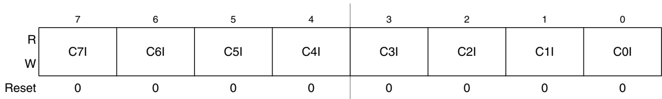
Figure 22-18. Timer Interrupt Enable Register (TIE)
