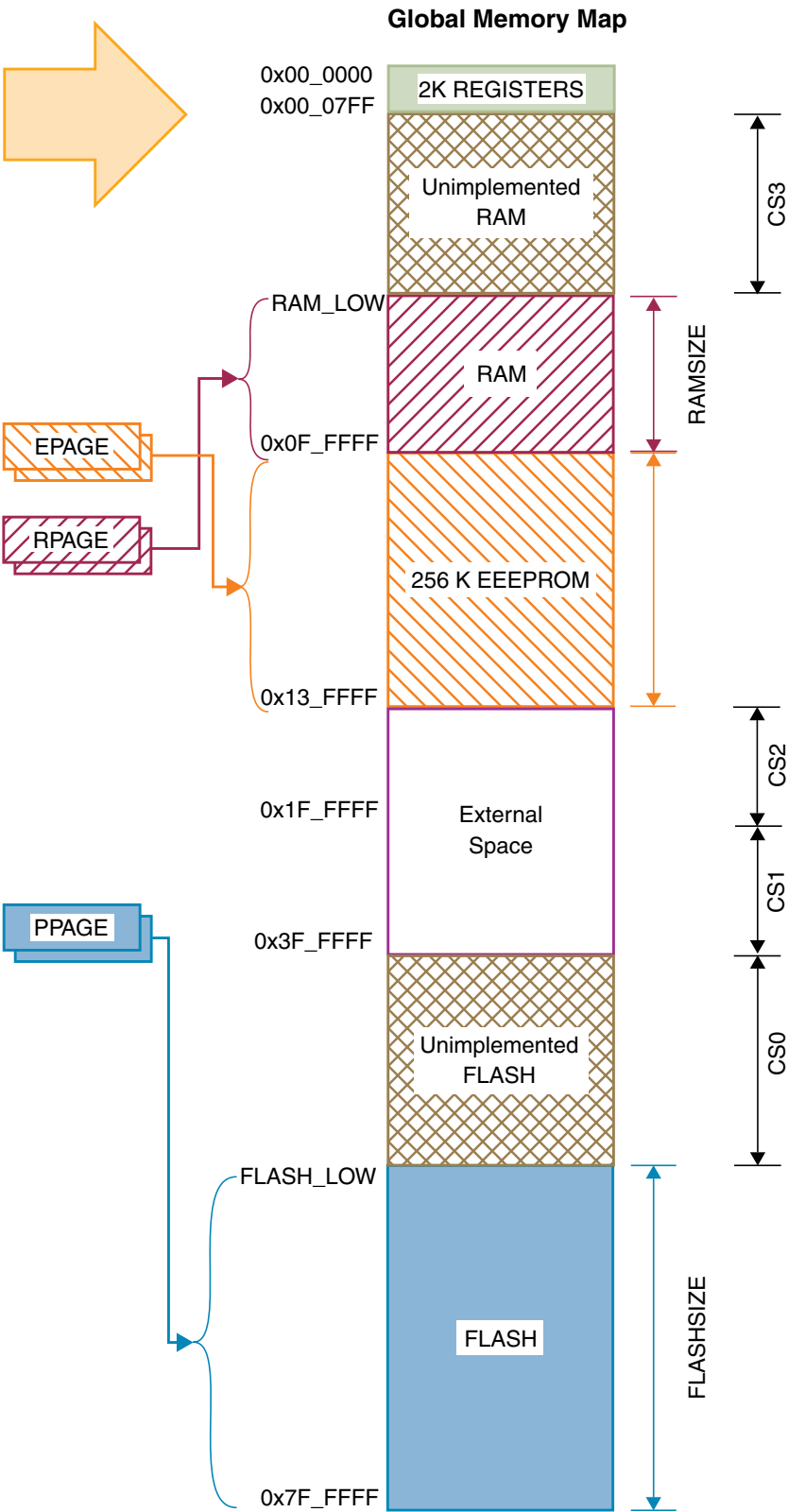
Figure 3-19. S12XE CPU & BDM Global Address Mapping
