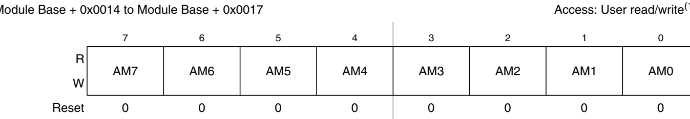
Figure 16-22. MSCAN Identifier Mask Registers (First Bank) — CANIDMR0–CANIDMR3
