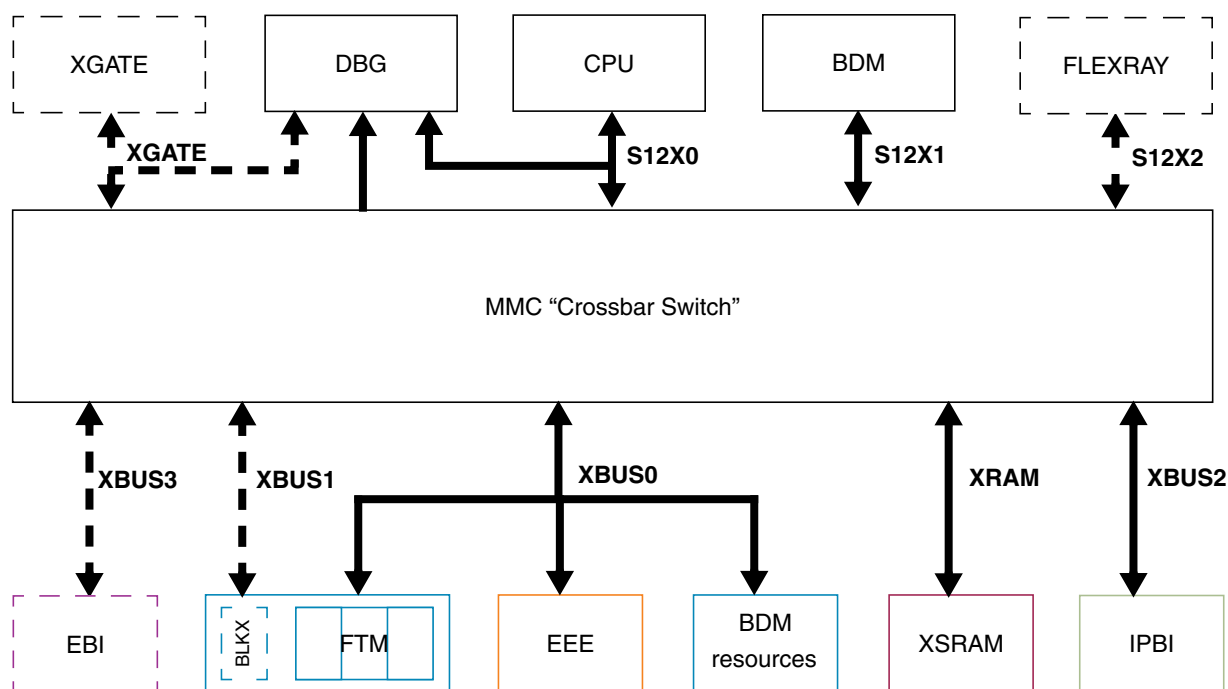
Figure 3-23. MMC Block Diagram
