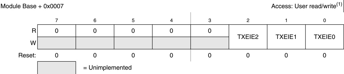
Figure 16-11. MSCAN Transmitter Interrupt Enable Register (CANTIER)
