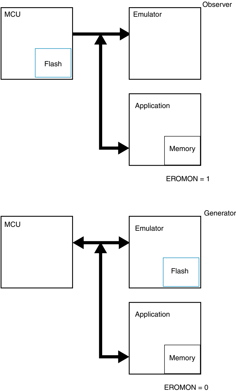
Figure 3-27. ROMON = 1 in Emulation Expanded Mode
