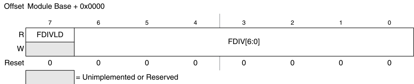
Figure 27-5. Flash Clock Divider Register (FCLKDIV)
