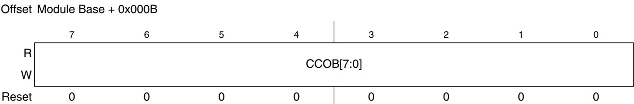
Figure 26-17. Flash Common Command Object Low Register (FCCOBLO)
