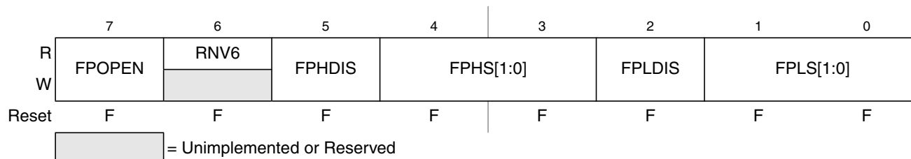
Figure 27-13. Flash Protection Register (FPROT)
