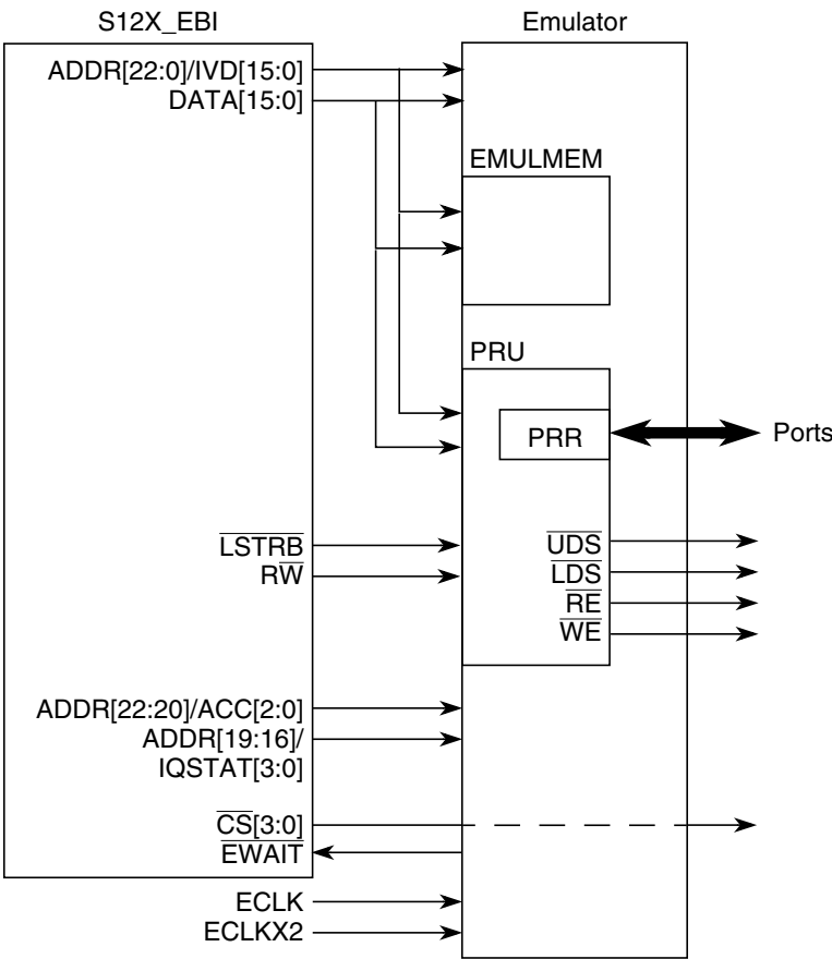
Figure 5-6. Application in Emulation Expanded Mode
