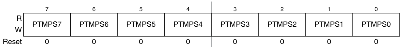
Figure 14-50. Precision Timer Modulus Counter Prescaler Select Register (PTMCPSR)
