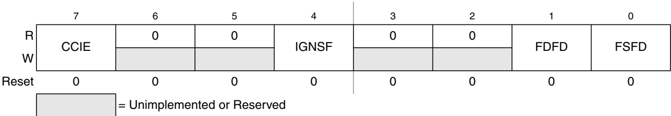
Figure 29-9. Flash Configuration Register (FCNFG)
