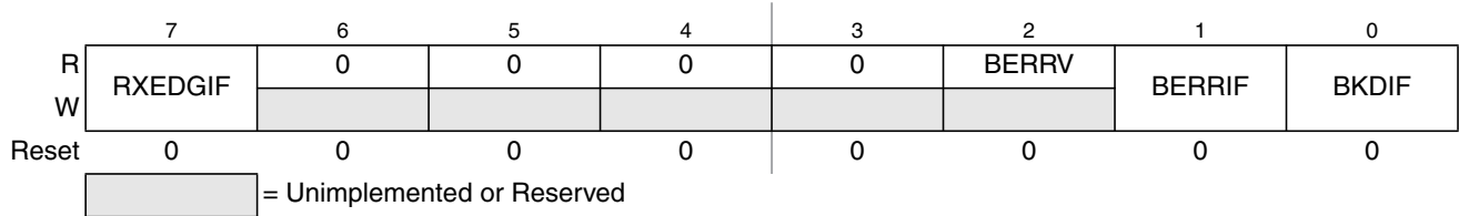
Figure 20-6. SCI Alternative Status Register 1 (SCIASR1)
