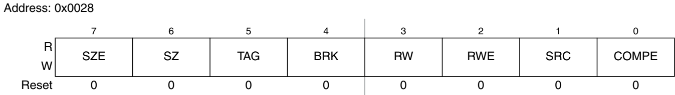
Figure 8-14. Debug Comparator Control Register (Comparators B and D)
