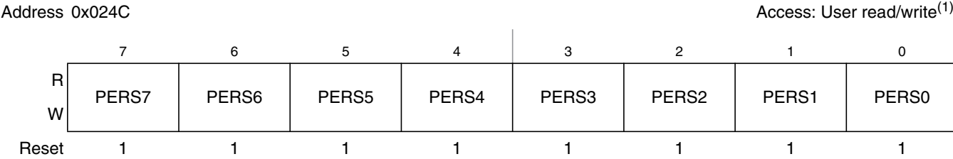
Figure 2-31. Port S Pull Device Enable Register (PERS)
