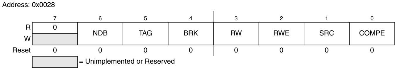
Figure 8-13. Debug Comparator Control Register (Comparators A and C)
