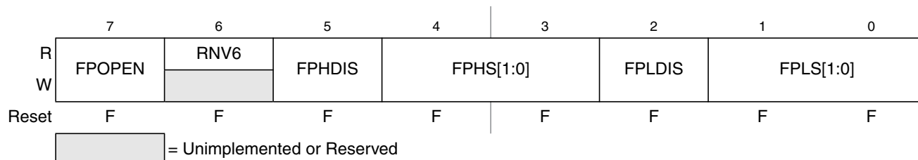
Figure 29-13. Flash Protection Register (FPROT)
