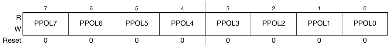
Figure 19-4. PWM Polarity Register (PWMPOL)
