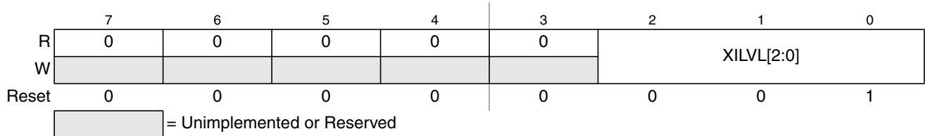
Figure 6-4. XGATE Interrupt Priority Configuration Register (INT_XGPRIOR)
