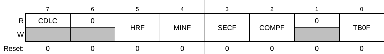
Figure 16-6. RTC Status and Control Register1 (RTCSC1)
