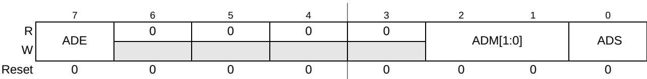
Figure 17-4. SSG attack/decay control register (SSGADC)
