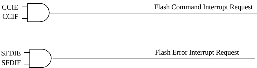
Figure 19-31. Flash Module Interrupts Implementation
