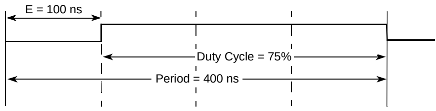
Figure 9-18. PWM Left Aligned Output Example Waveform
