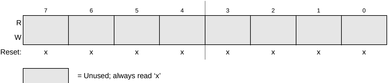
Figure 11-33. Identifier Register 3 — Standard Mapping
