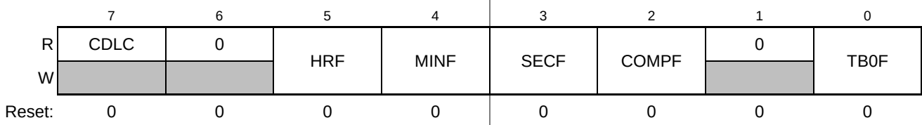
Figure 16-6. RTC Status and Control Register1 (RTCSC1)
