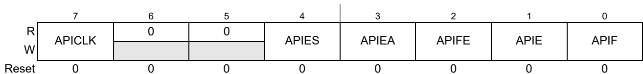
Figure 10-17. Autonomous Periodical Interrupt Control Register (CPMUAPICTL)
