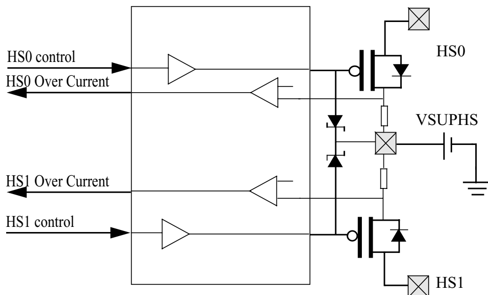
Figure 13-1. HSDRV Block Diagram
