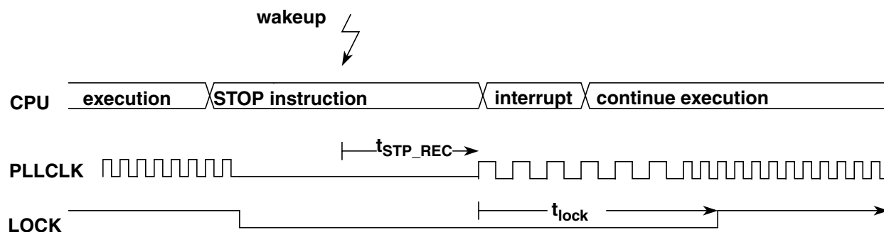
Figure 4-34. Stop Mode using PLLCLK as source of the Bus Clock
