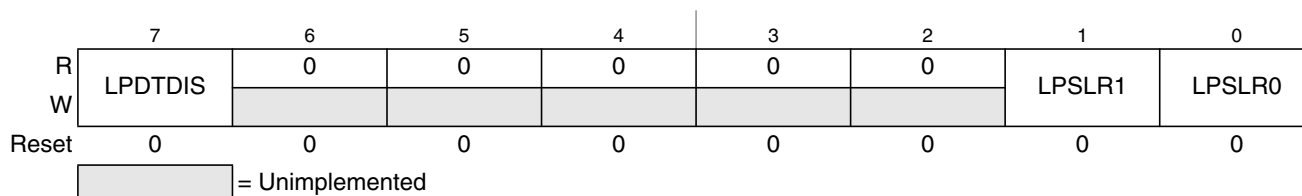
Figure 15-6. LIN Slew Rate Mode Register (LPSLRM)
