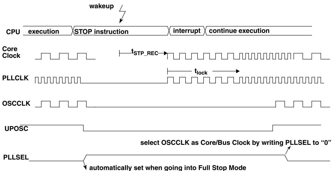
Figure 4-35. Full Stop Mode using Oscillator Clock as source of the Bus Clock
