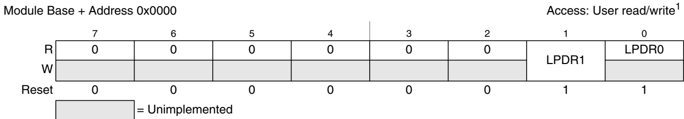
Figure 15-3. Port LP Data Register (LPDR)
