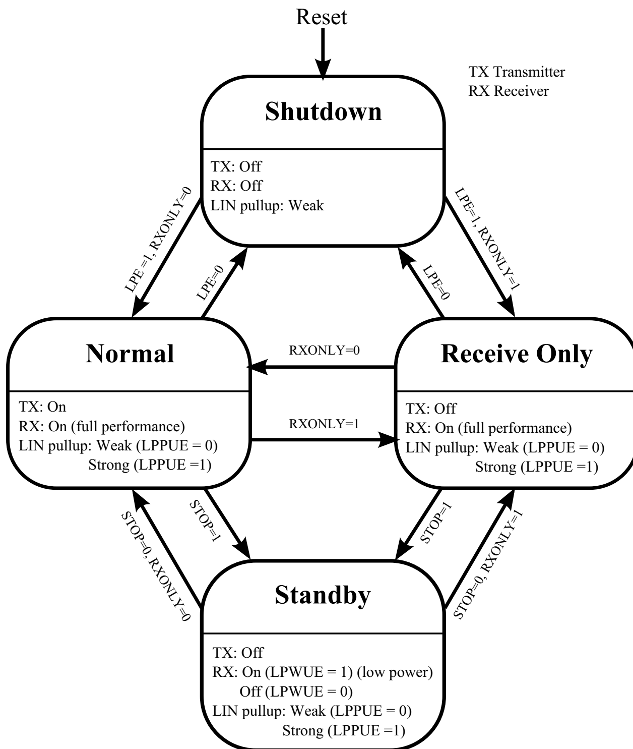
Figure 15-11. LIN Physical Layer Mode Transitions
