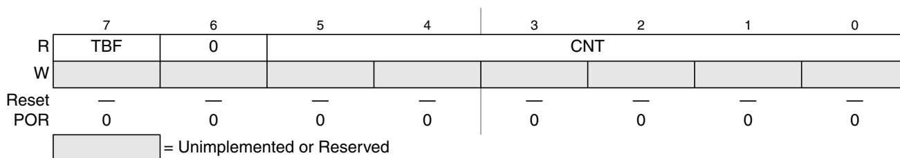
Figure 6-8. Debug Count Register (DBGCNT)
