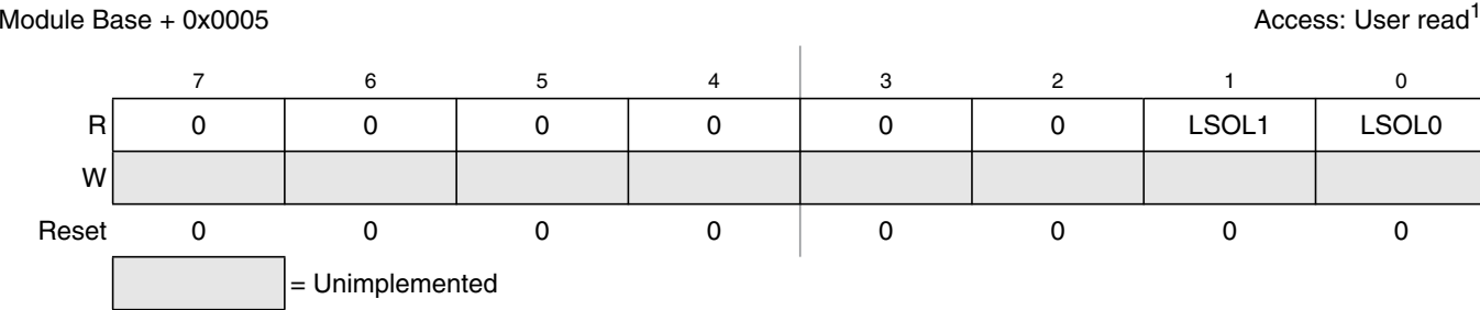
Figure 14-4. LSDRV Status Register (LSSR)
