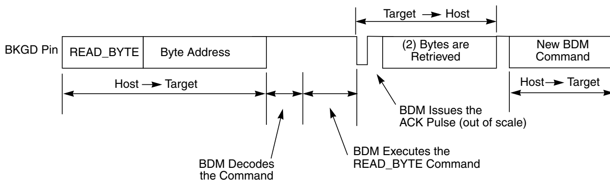
Figure 5-11. Handshake Protocol at Command Level
