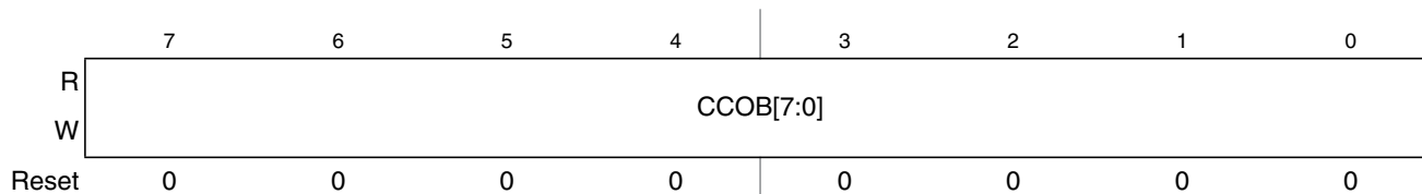
Figure 17-16. Flash Common Command Object Low Register (FCCOBLO)
