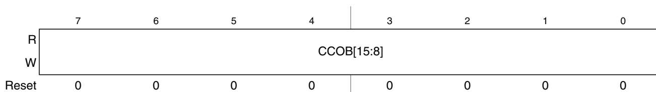
Figure 17-15. Flash Common Command Object High Register (FCCOBHI)
