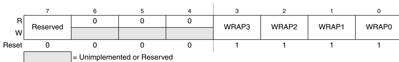
Figure 8-3. ATD Control Register 0 (ATDCTL0)
