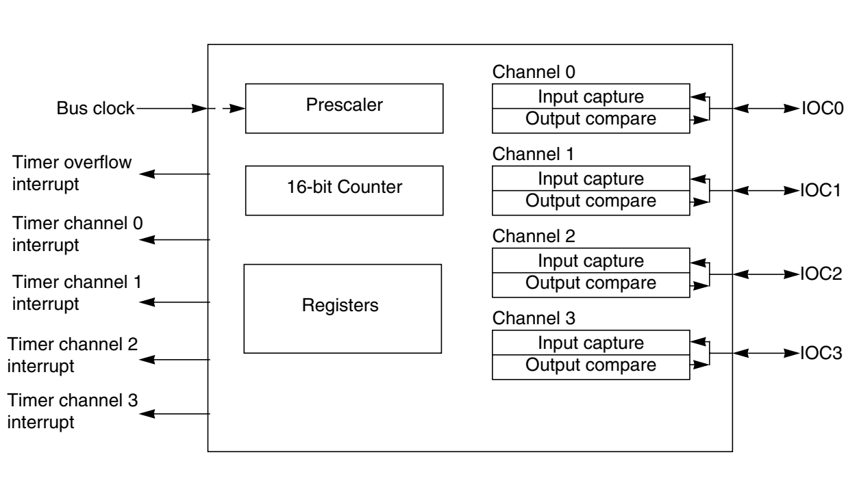
Figure 12-1. TIM16B4CV3 Block Diagram
