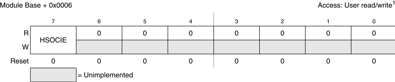
Figure 13-5. HSDRV Interrupt Enable Register (HSIE)
