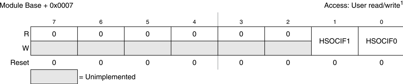
Figure 13-6. HSDRV Interrupt Flag Register (HSIF)
