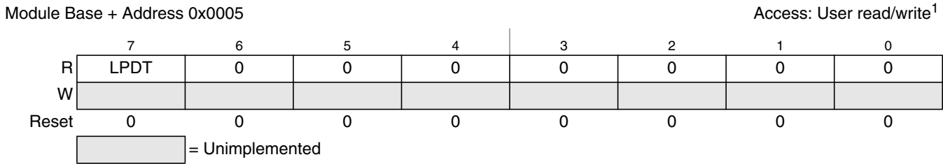
Figure 15-8. LIN Status Register (LPSR)
