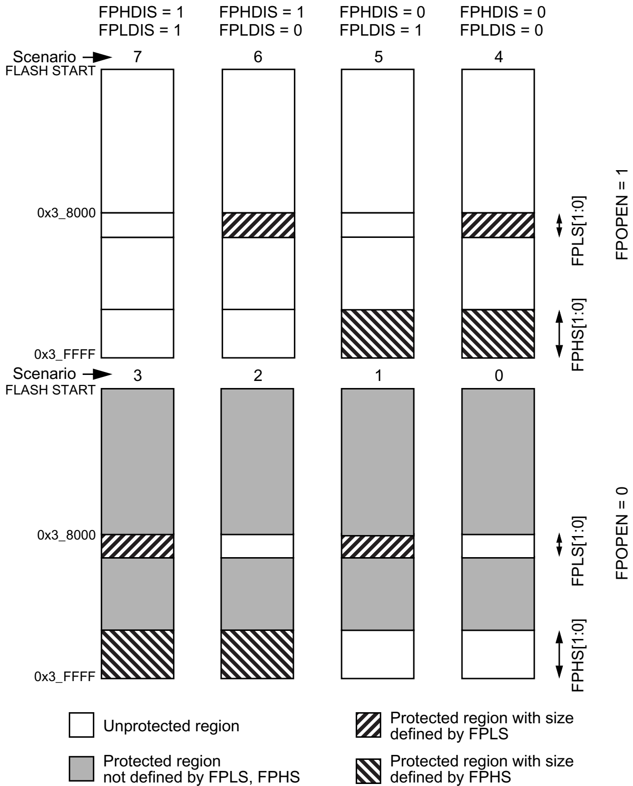
Figure 17-13. P-Flash Protection Scenarios
