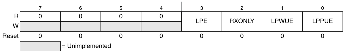
Figure 15-4. LIN Control Register (LPCR)
