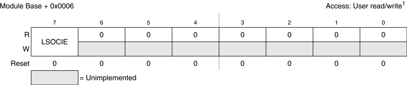
Figure 14-5. LSDRV Interrupt Enable Register (LSIE)
