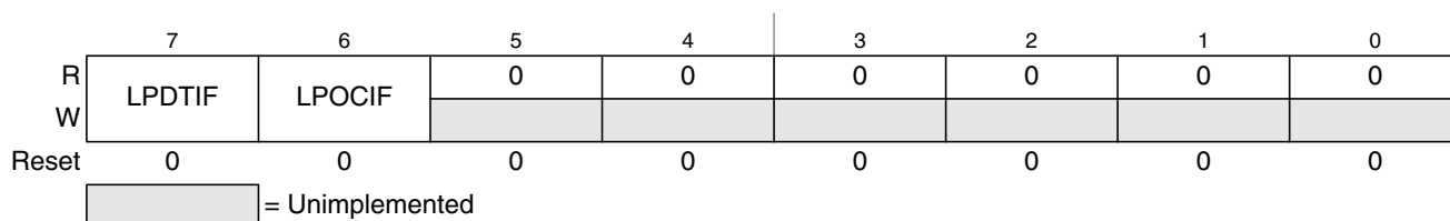
Figure 15-10. LIN Interrupt Flags Register (LPIF)
