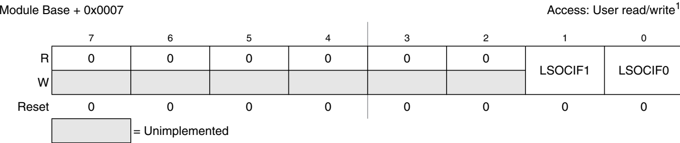
Figure 14-6. LSDRV Interrupt Flag Register (LSIF)
