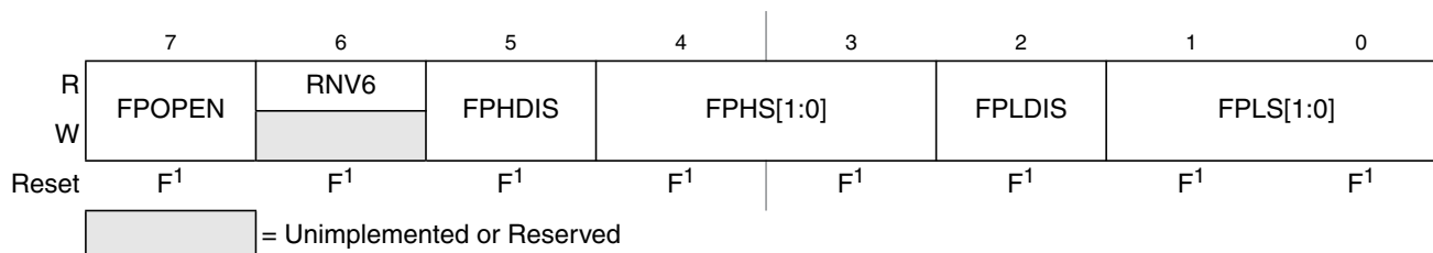
Figure 17-12. Flash Protection Register (FPROT)
