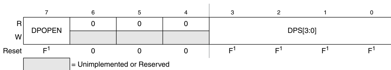
Figure 17-14. EEPROM Protection Register (EEPROT)
