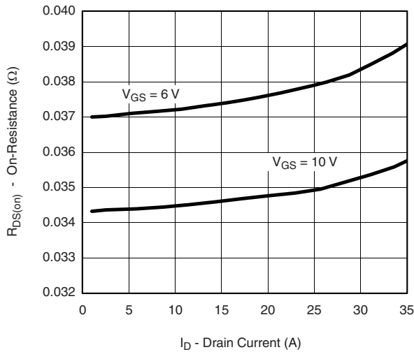
V_{GS} = 6\text{ V} V_{GS} = 10\text{ V} On-Resistance vs. Drain Current and Gate Voltage
