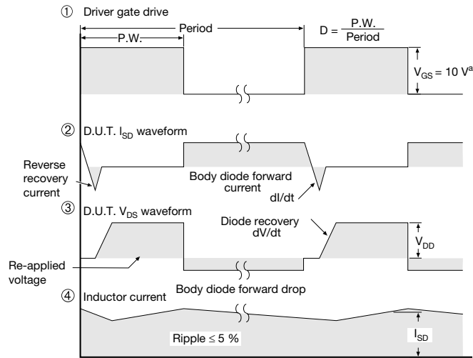
Fig. 20 - For N-Channel
