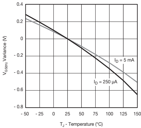
Threshold Voltage
