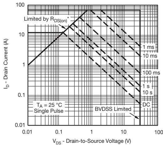
* V_{DS} > minimum V_{DS} at which R_{DS(on)} is specified Safe Operating Area, Junction-to-Ambient
