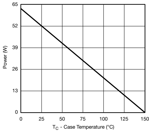
Power, Junction-to-Case
