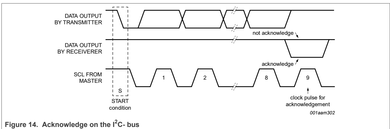
Figure 14. Acknowledge on the I 2 C- bus
