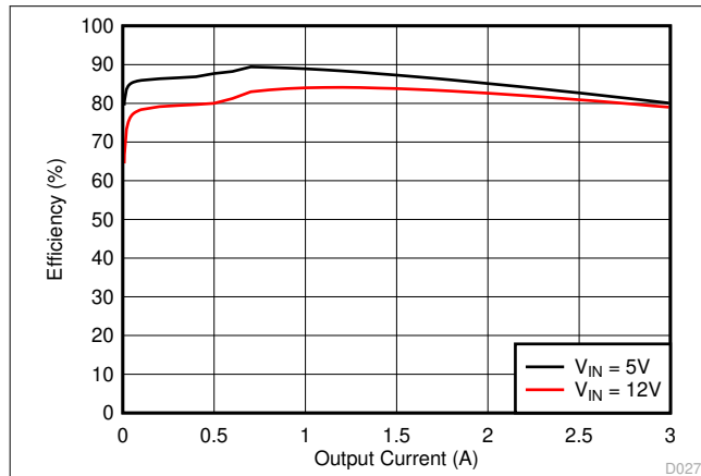
Figure 8-17. Tps563200 Efficiency
