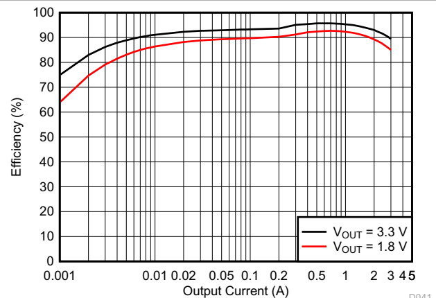
Figure 6-15. Efficiency vs Output Current
