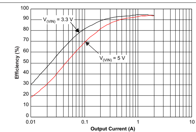
Figure 36. Efficiency versus Load Current
