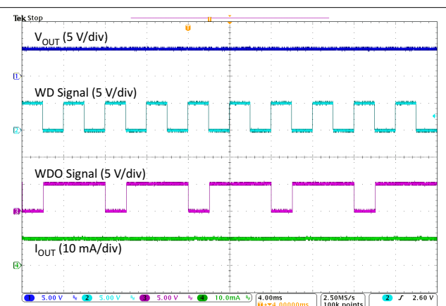
Figure 8-3. TPS7B6350-Q1 Watchdog Fault (High-Frequency Watchdog Service Signal)
