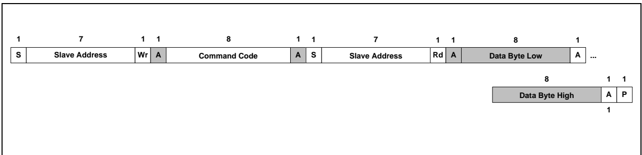
Figure 31: SMBus Read Word Protocol
