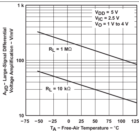
Figure 23. Large-Signal Differential Voltage Amplification vs Ambient Temperature
