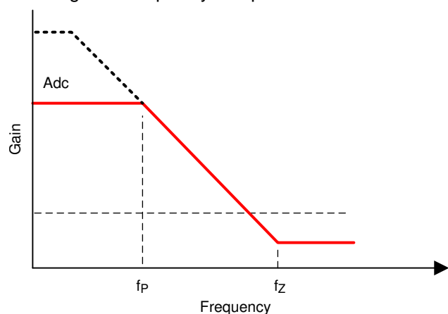
Figure 33. Frequency Response
