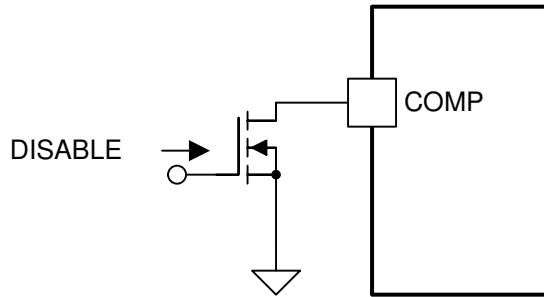
Figure 8-7. Disable Circuit
