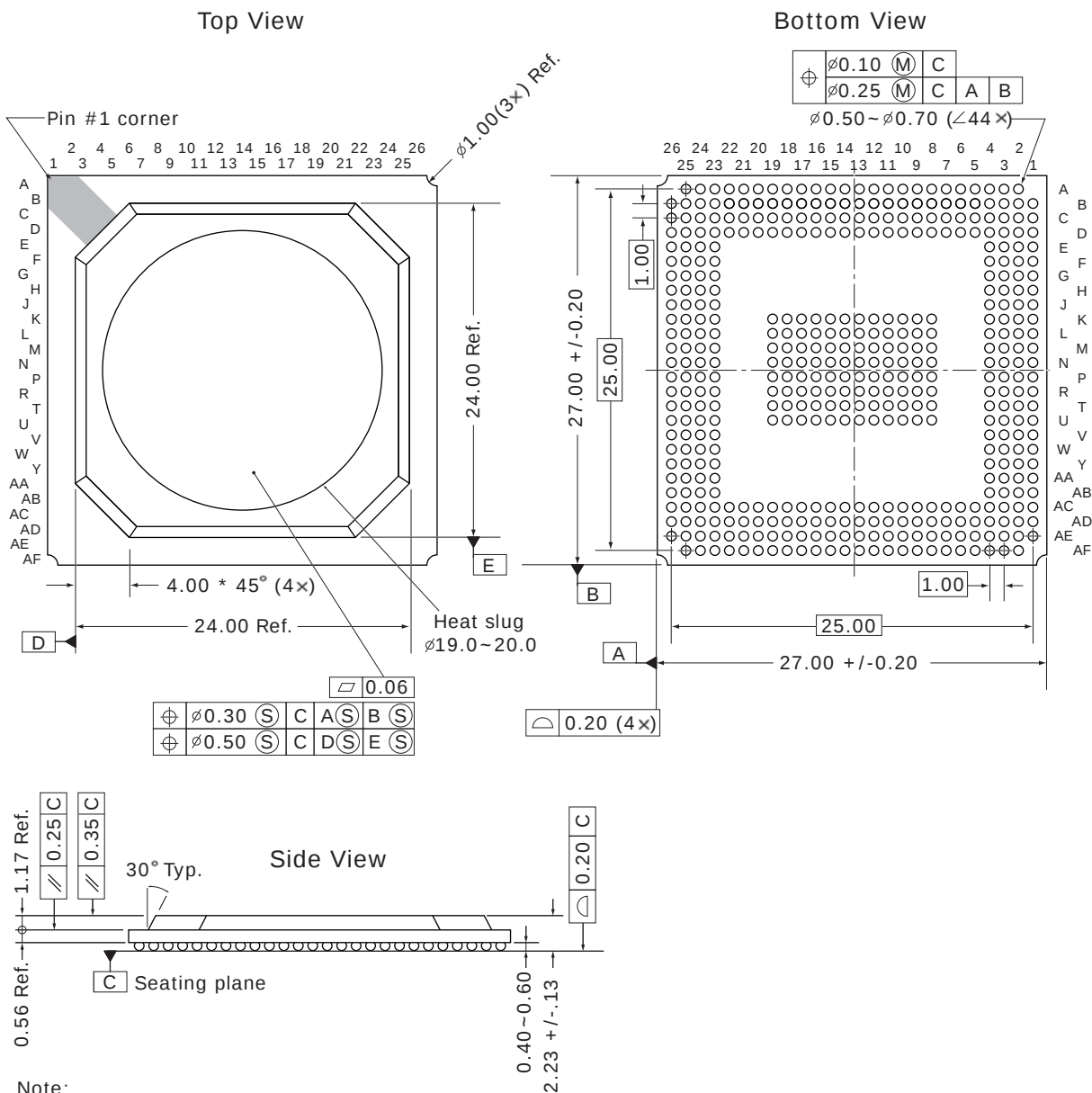
Figure 25 • Package Drawing
