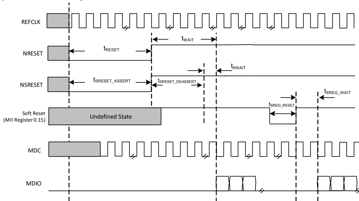
Figure 21 • Reset Timing
