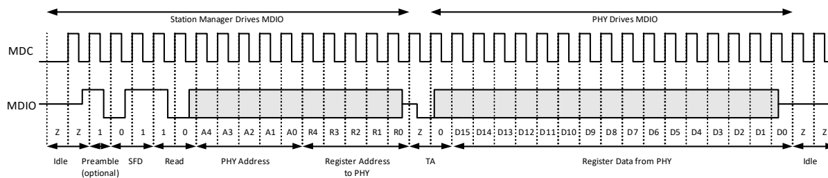
Figure 9 • SMI Read Frame
