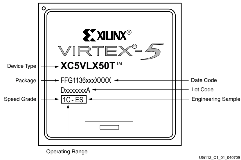
Figure 1-1: Top Marking (for Large Device Packages)
