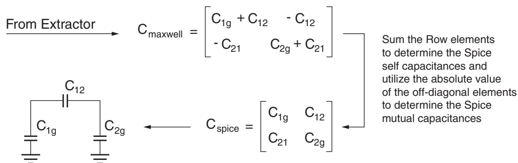
Figure 4-8: Maxwellian and Spice-Formatted Matrices (2 x 2 matrix)
