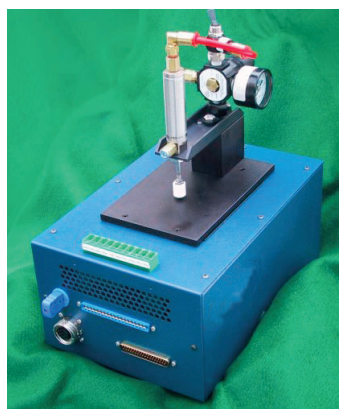
Figure 3-9: \theta_{JC} Measurement Setup
