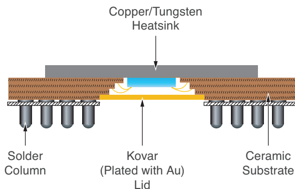
Figure 1-9: CG560 Package
