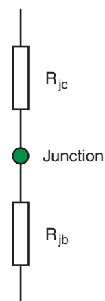
Two-Resistor Model
