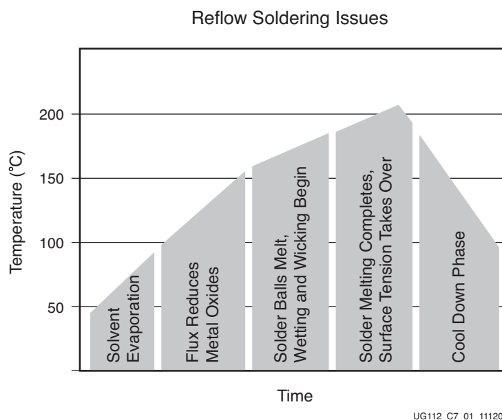
Figure 7-1: Soldering Sequence
