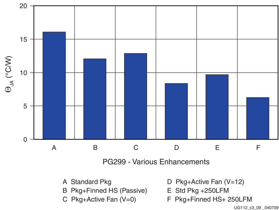
Figure 3-5: Effect of Active and Passive Heat Sinks on the Thermal Resistance (θ JA ) of PG299 Packages
