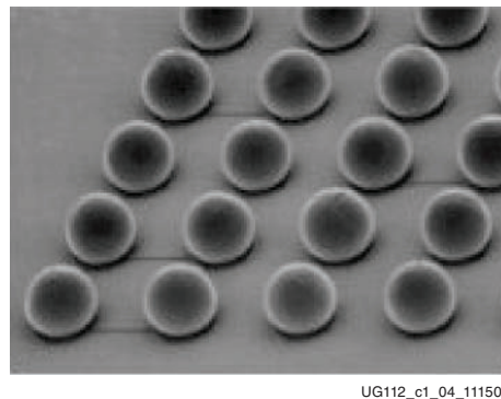
Figure 1-4: Eutectic Bumps
