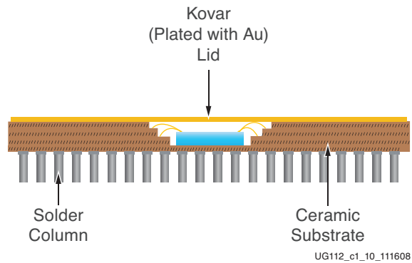
Figure 1-10: CG717 Package
