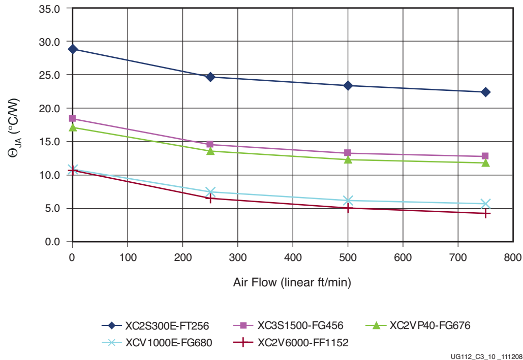
Figure 3-6: Effect of Air Flow on the Thermal Resistance (θ JA ) of BGA Packages
