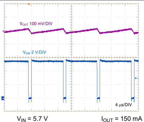
V_{IN} = 5.7\text{ V} I_{OUT} = 150\text{ mA} Figure 8-7. SW Node and Output Ripple Voltage Showing Frequency Foldback Near Dropout
