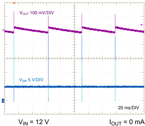
V_{IN} = 12\text{ V} I_{OUT} = 0\text{ mA} Figure 8-5. SW Node and Output Ripple Voltage, No Load
