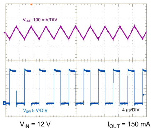
V_{IN} = 12\text{ V} I_{OUT} = 150\text{ mA} Figure 8-6. SW Node and Output Ripple Voltage, Full Load
