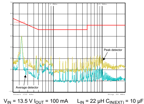
V_{IN} = 13.5\text{ V} I_{OUT} = 100\text{ mA} L_{IN} = 22\text{ }\mu\text{H} C_{IN(EXT)} = 10\text{ }\mu\text{F} Figure 8-4. EMI Plot – CISPR 22 Filtered Emissions
