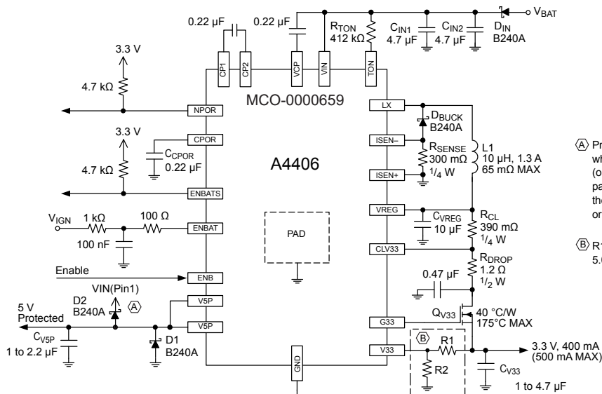
Option with external LDO set to 3.3 V / 400 mA, (Add R1 and R2 and remove R DRIP to set external LDO to 5.0 V / 400 mA)
