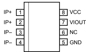
Package OL, 8-Pin SOIC Pinout Diagram
