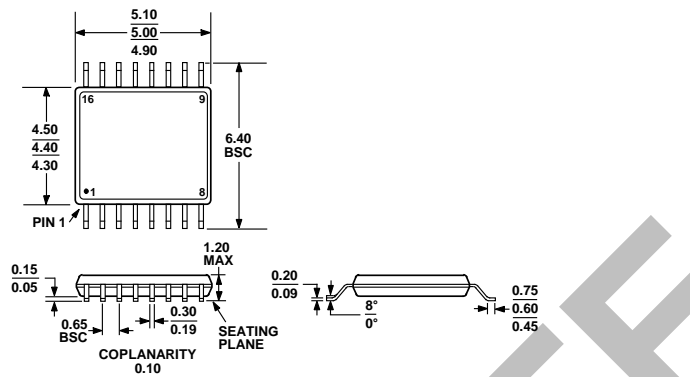
COMPLIANT TO JEDEC STANDARDS MO-153-AB Figure 20. 16-Lead Thin Shrink Small Outline Package [TSSOP] (RU-16) Dimensions shown in millimeters
