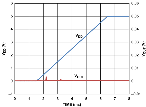
Figure 41. Power-On Reset to 0 V
