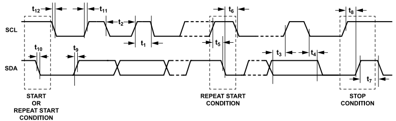
Figure 3. I 2 C Serial Interface Timing Diagram
