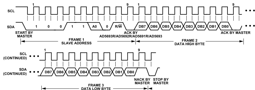
Figure 49. I 2 C Read Operation
