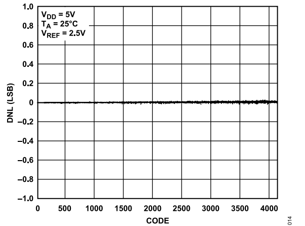
Figure 14. AD5691R DNL
