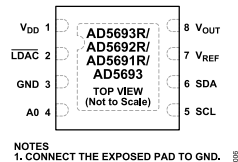
Figure 6. AD5693R/AD5692R/AD5691R/AD5693 Pin Configuration, 8-Lead LFCSP, LDAC Option
