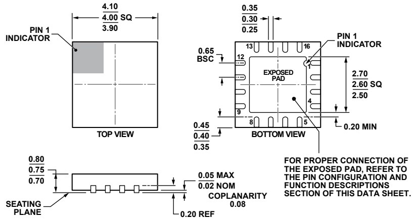
Figure 63. 16-Lead Lead Frame Chip Scale Package [LFCSQ_WQ] 4 mm × 4 mm Body, Very Very Thin Quad (CP-16-17) Dimensions shown in millimeters
