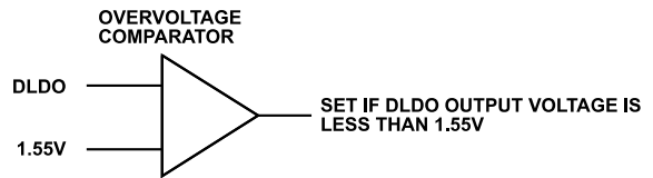
Figure 122. Digital LDO Monitor
