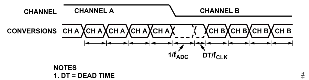
Figure 105. Fast Settling, Sinc 3 + Sinc 1 Filter
