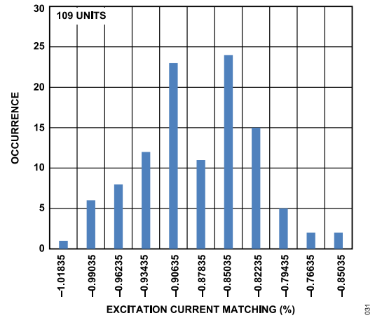
Figure 32. IOUTx Current Initial Matching Histogram (500 µA)
