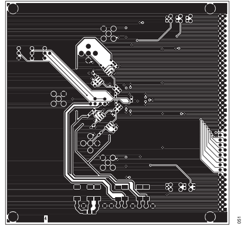
Figure 51. Bottom Routing
