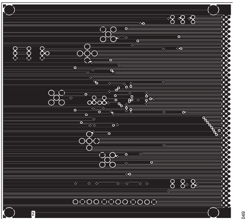
Figure 49. Ground Plane
