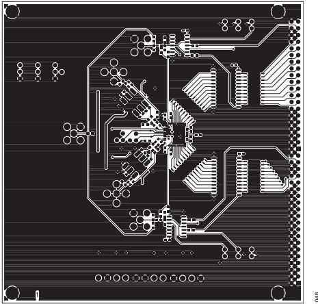
Figure 48. Top Routing
