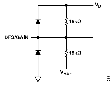
Figure 13. DFS/Gain Input
