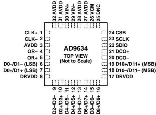
Figure 3. Pin Configuration
