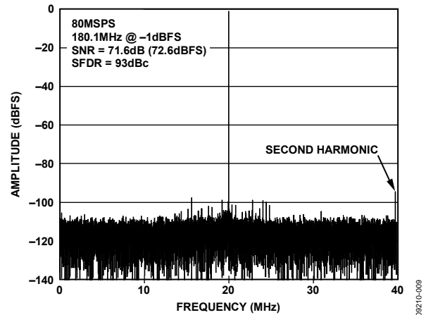
Figure 9. AD9641-80 Single-Tone FFT with f_{IN} = 180.1 MHz
