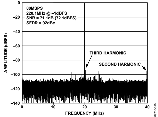
Figure 10. AD9641-80 Single-Tone FFT with f_{IN} = 220.1 MHz
