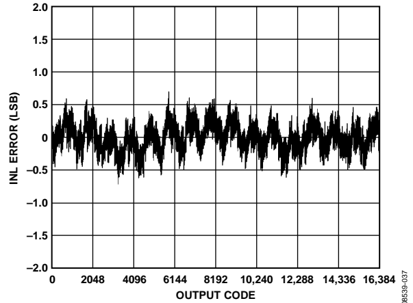
Figure 15. AD9649-80 INL Error with f_{IN} = 9.7 MHz
