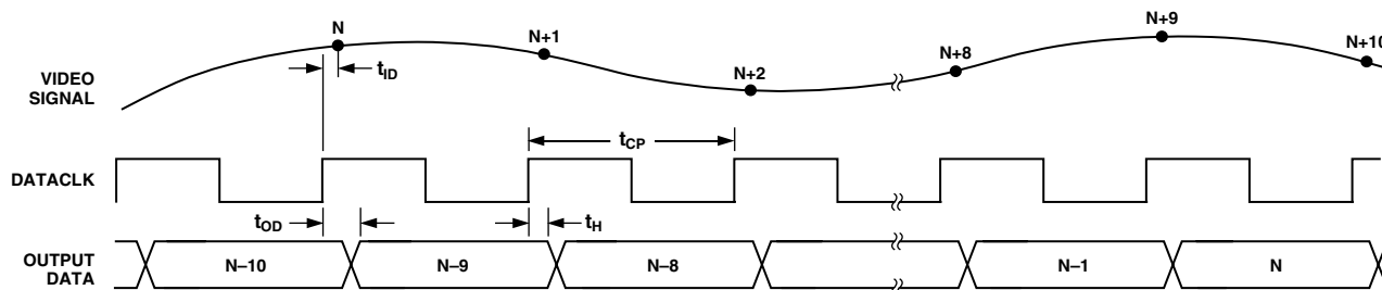
Figure 7. AUX-Mode Timing
