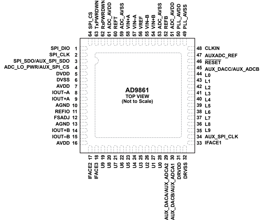
Figure 3. Pin Configuration
