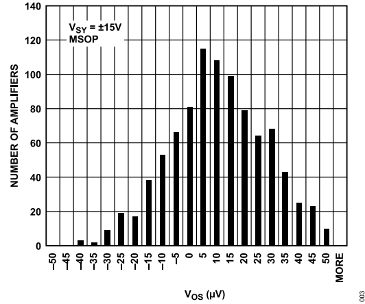
Figure 13. ADA4077-2 Offset Voltage ( V_{OS} ) Distribution, V_{SY} = \pm 15\text{ V}
