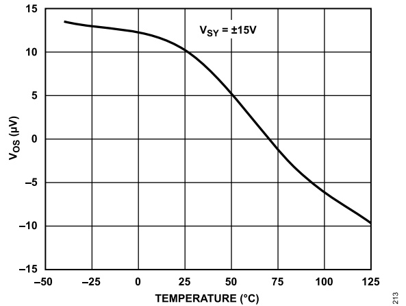
Figure 15. Offset Voltage ( V_{OS} ) vs. Temperature, V_{SY} = \pm 15\text{ V}
