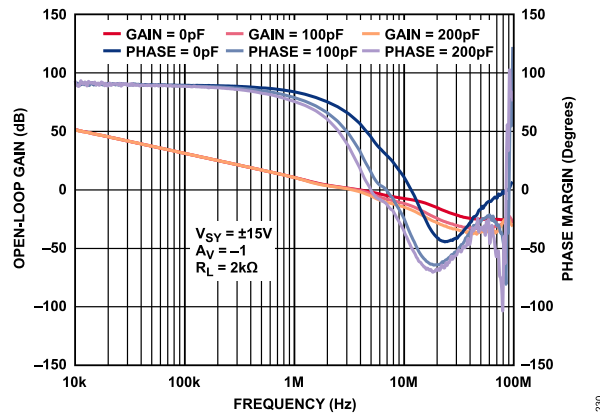
Figure 33. Open-Loop Gain and Phase Margin vs. Frequency, V_{SY} = \pm 15 V
